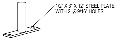
☐ SURFACE FLANGE MOUNT (SF)
