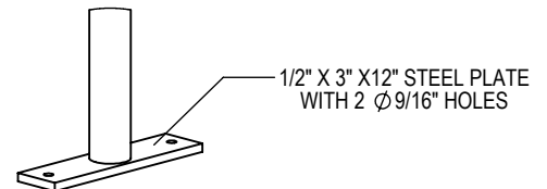
□ SURFACE FLANGE MOUNT (SF)
