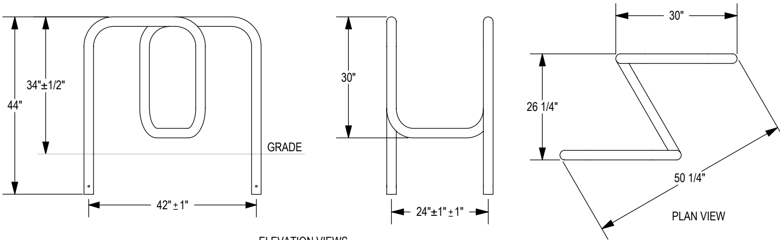
ELEVATION VIEWS 2 HOOP - 4 BIKE
