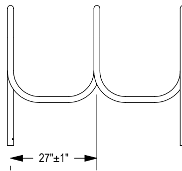
ELEVATION VIEWS 3 HOOP - 6 BIKE CAPACITY
