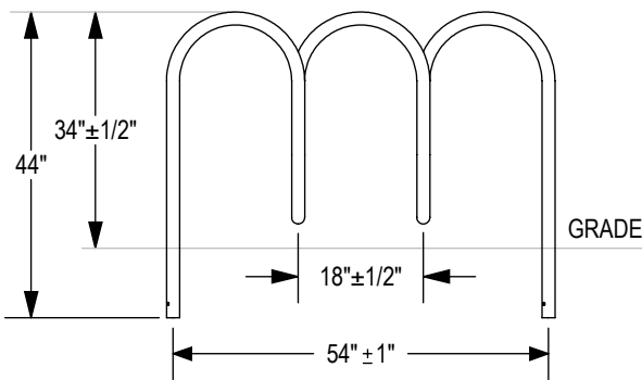
ELEVATION VIEWS 3 HOOP - 6 BIKE CAPACITY
